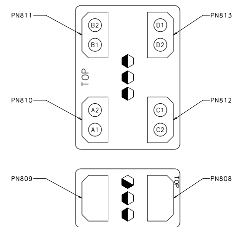
CONNECTOR KEYING AND CONN LOCATION (FRONT VIEW OF RACK CONNECTOR)
